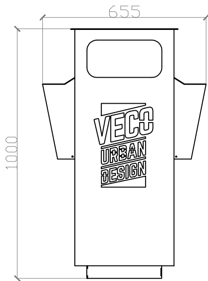
VISTA FRONTAL
