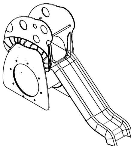
VISTA ISOMÉTRICA ISOMETRIC VIEW
