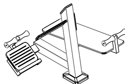
VISTA ISOMÉTRICA ISOMETRIC VIEW
