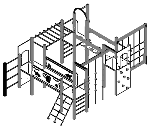
VISTA ISOMÉTRICA ISOMETRIC VIEW
