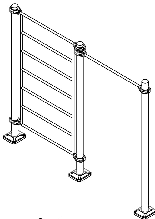
VISTA ISOMÉTRICA ISOMETRIC VIEW
