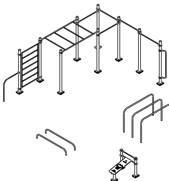
VISTA ISOMÉTRICA ISOMETRIC VIEW
