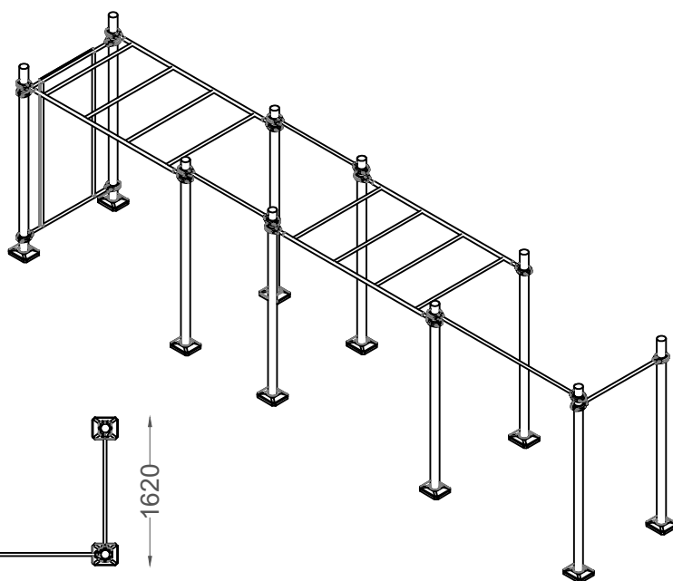
VISTA ISOMÉTRICA ISOMETRIC VIEW
