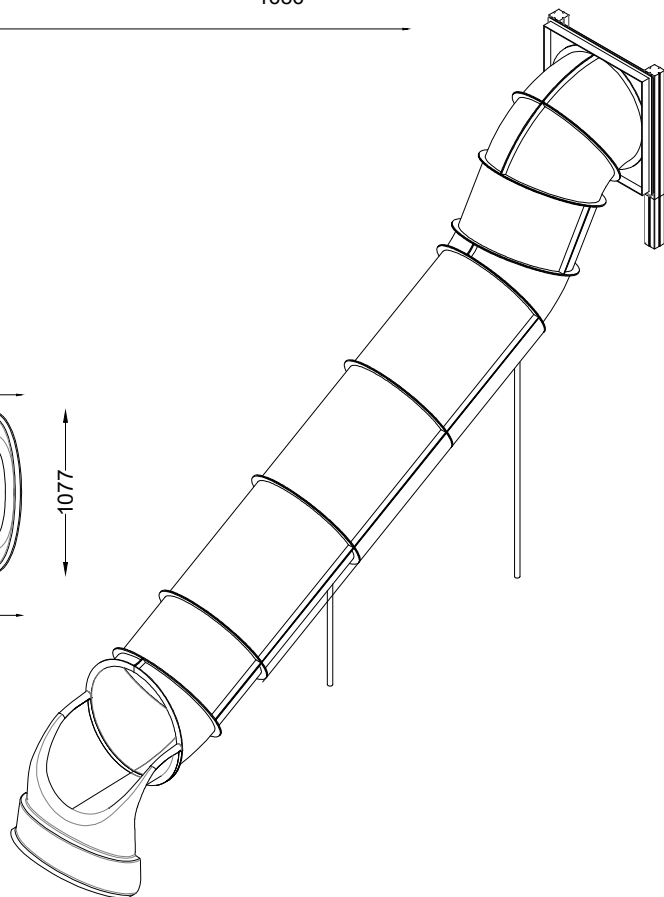
VISTA ISOMÉTRICA ISOMETRIC VIEW
