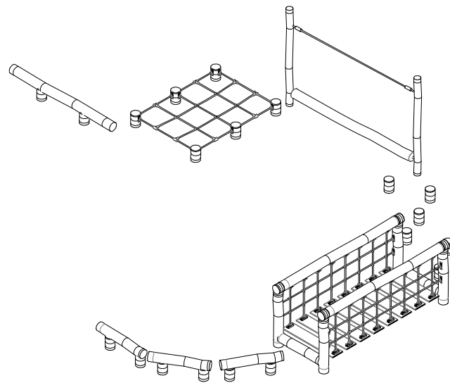
VISTA ISOMÉTRICA ISOMETRIC VIEW
