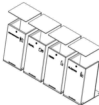
VISTA ISOMÉTRICA ISOMETRIC VIEW
