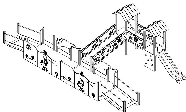
VISTA ISOMÉTRICA ISOMETRIC VIEW
