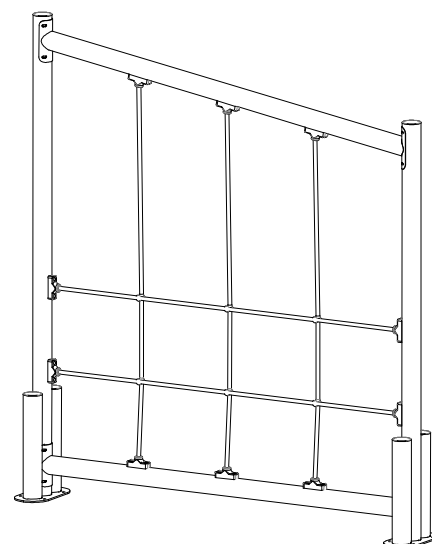
VISTA ISOMÉTRICA ISOMETRIC VIEW
