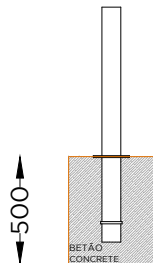
MACIÇO BETÃO P/ENTERRAMENTO CONCRETE BLOCK BY BURIAL
