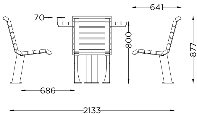
ALÇADO FRONTAL/ LATERAL FRONT/ SIDE VIEW
