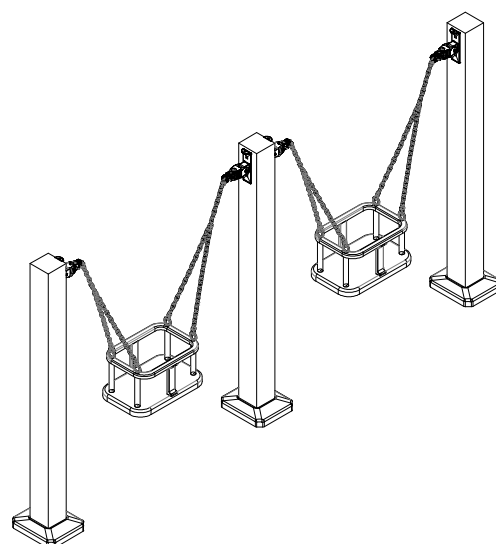
VISTA ISOMÉTRICA ISOMETRIC VIEW
