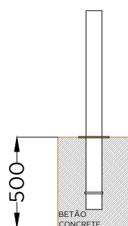
MACIÇO BETÃO P/ENTERRAMENTO CONCRETE BLOCK BY BURIAL
