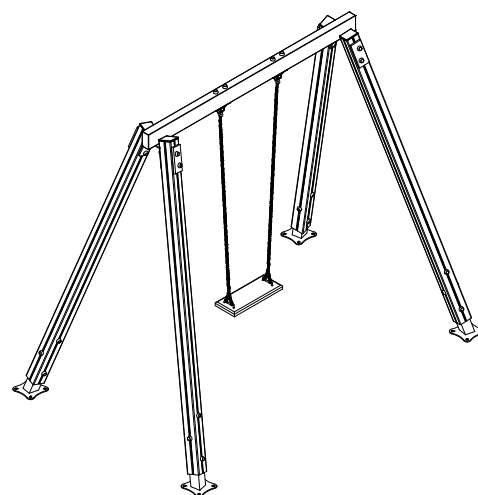
VISTA ISOMÉTRICA ISOMETRIC VIEW
