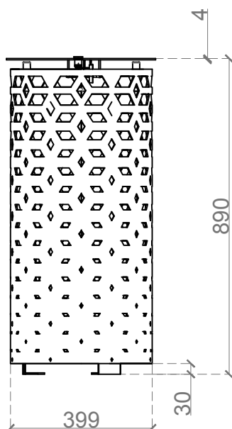
VISTA FRONTAL
