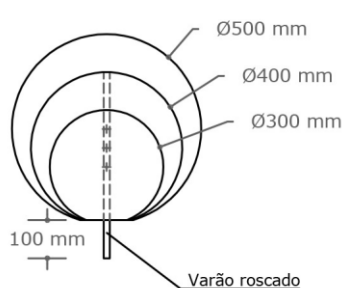
Alçado Frontal/Lateral Front/Lateral View
