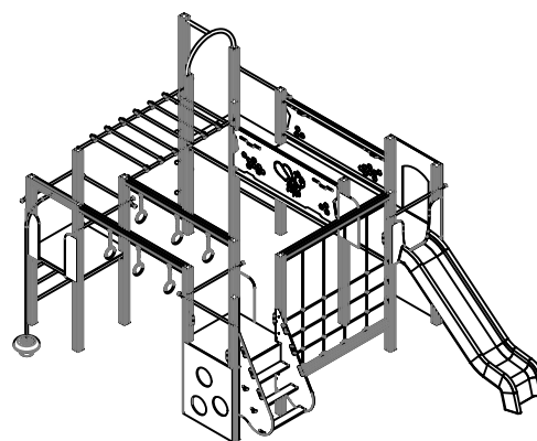
VISTA ISOMÉTRICA ISOMETRIC VIEW
