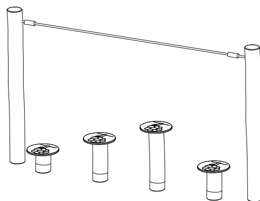
VISTA ISOMÉTRICA ISOMETRIC VIEW
