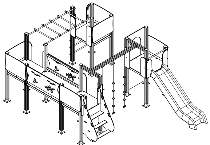
VISTA ISOMÉTRICA ISOMETRIC VIEW
