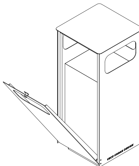
VISTA ISOMÉTRICA ISOMETRIC VIEW
