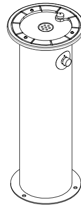
VISTA ISOMÉTRICA ISOMETRIC VIEW
