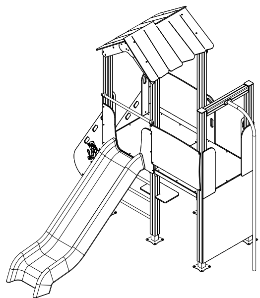
VISTA ISOMÉTRICA ISOMETRIC VIEW
