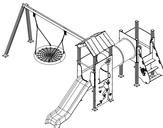
VISTA ISOMÉTRICA ISOMETRIC VIEW
