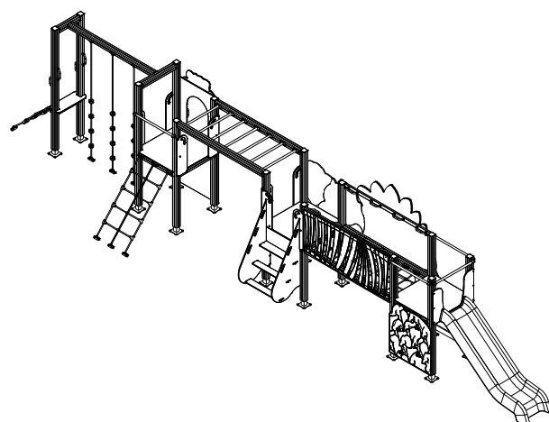
VISTA ISOMÉTRICA ISOMETRIC VIEW
