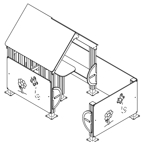
VISTA ISOMÉTRICA ISOMETRIC VIEW
