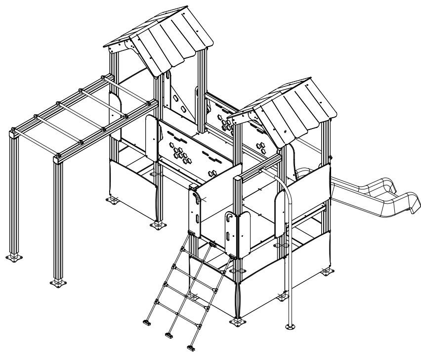
VISTA ISOMÉTRICA ISOMETRIC VIEW
