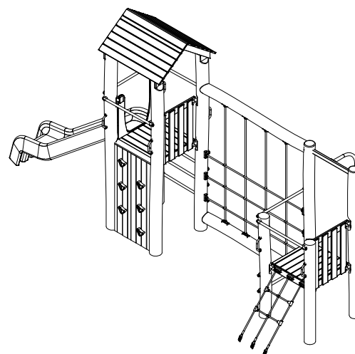
VISTA ISOMÉTRICA ISOMETRIC VIEW
